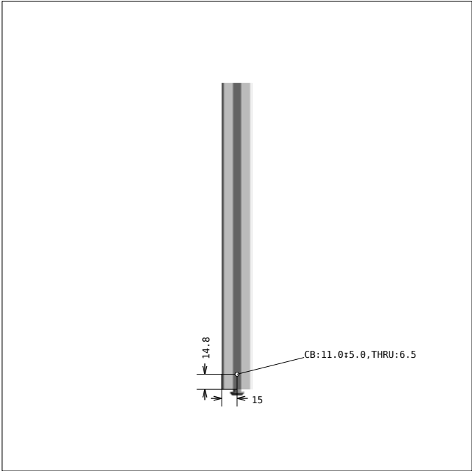
DRAWING 2, Pos 4 SIDE 2
