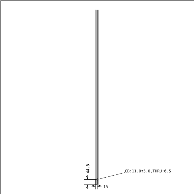
DRAWING 1, Pos 2 SIDE 1, bar length: 1500.0 mm
